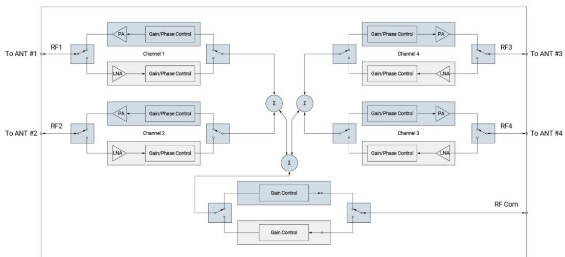
Figure 2. 5G Beamformer System Diagram (4 channels)
